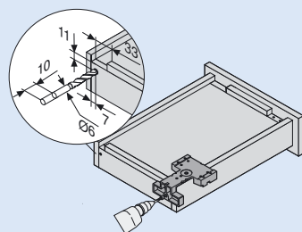
Drawer drilling jig (Hook)
