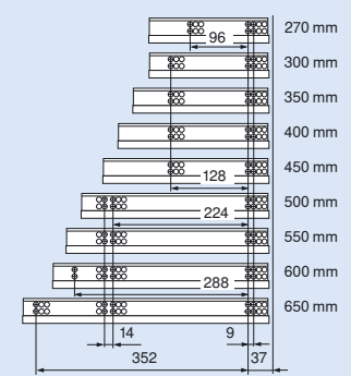
Hole pattern 550H
