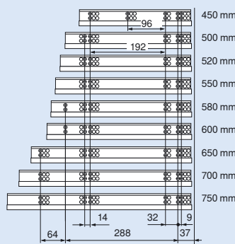
Hole pattern 566H
