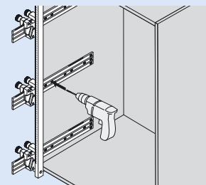
Universal drilling template Also available as an individual template (65.1051)
