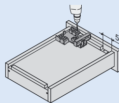
Drawer drilling jig (Locking device)
