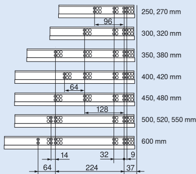
Hole pattern 560H
