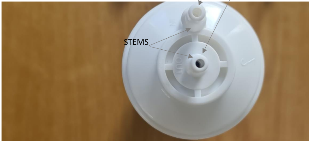
Figure 5. Push smaller diameter of elbow push fit fittings fully on to the IN and OUT stems of the filter (will feel click when fully inserted into position on the filter) as shown below
